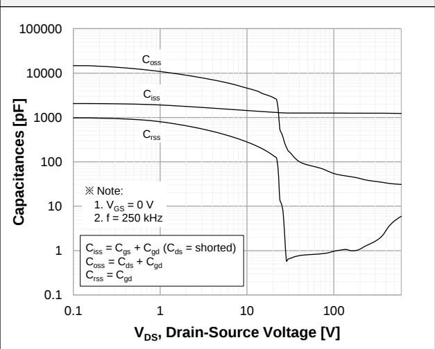
Figure 5. Capacitance Characteristics
