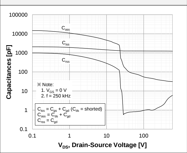
Figure 5. Capacitance Characteristics
